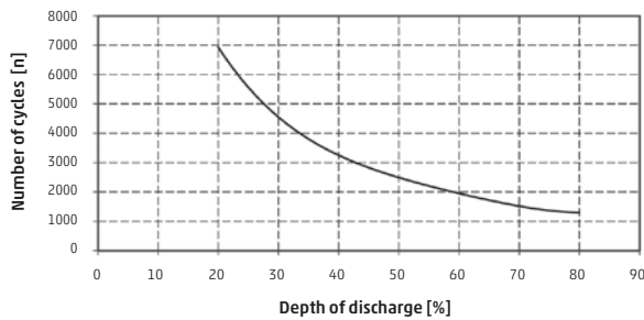
Fig. A Series OPzV bloc
